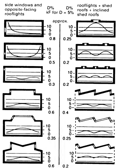
kF = \text{window area/floor area} = 1.6 values required for D_{min} = 5\% are shown for comparison
